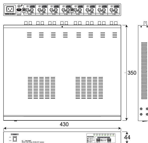
[ HEX-108D4M ]
