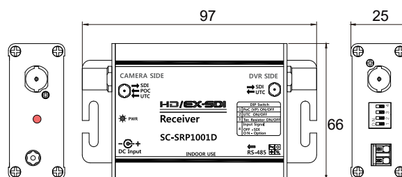
[ HEX-101D4M ]
