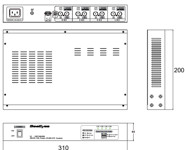
[ HEX-104D4M ]
